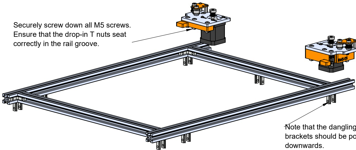
Exploded View
